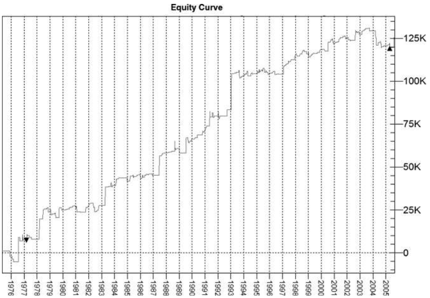
FIGURE 19.3 Equity curve.
